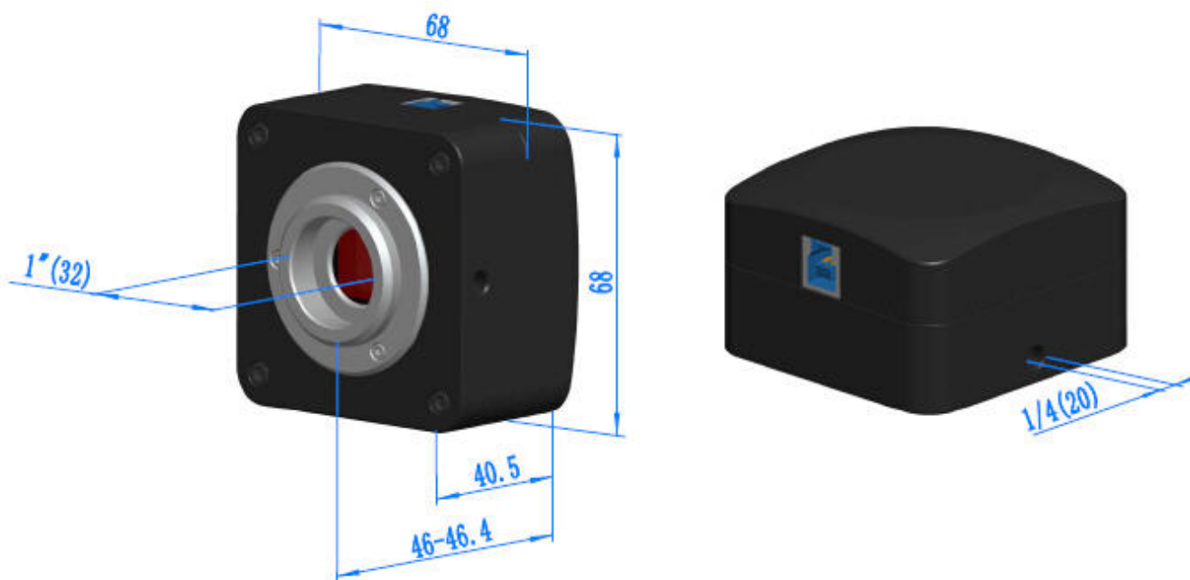
Dimension of E3ISPM Series Camera
