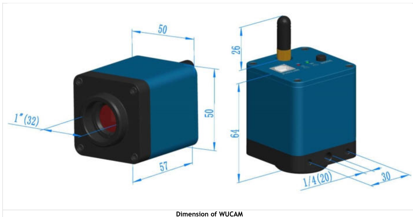
Dimension of WUCAM
